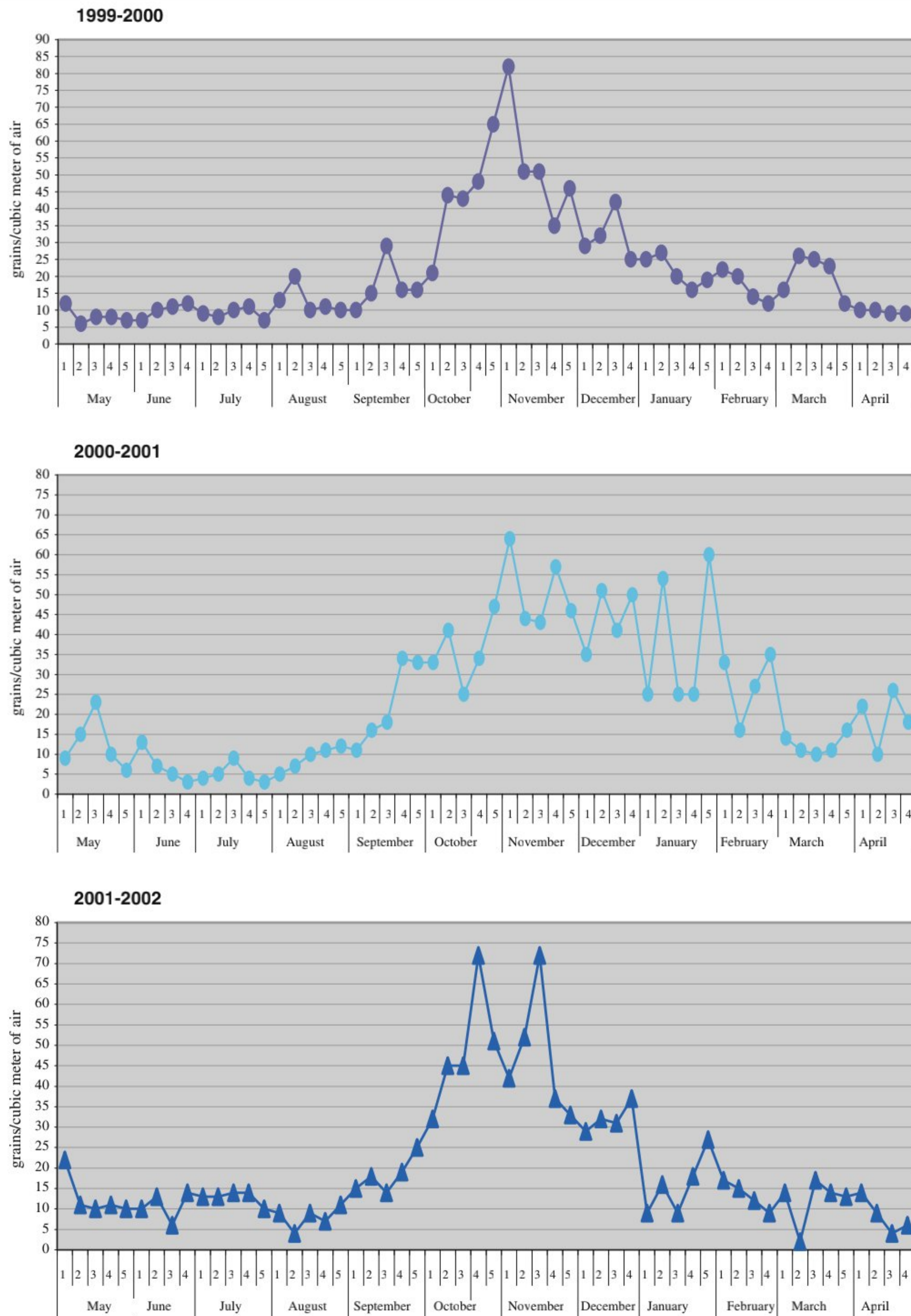
Fig. 1 Weekly Parietaria judaica pollen concentrations average between 1999–2000, 2000–2001, and 2001–2002
